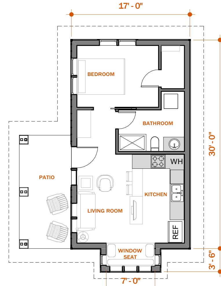
FLOOR PLAN
